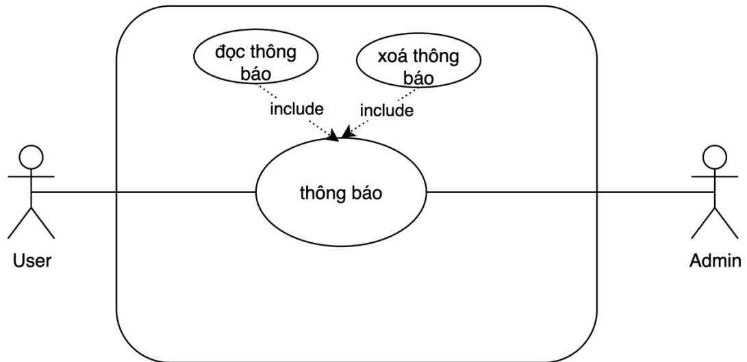
UC_Notification.
