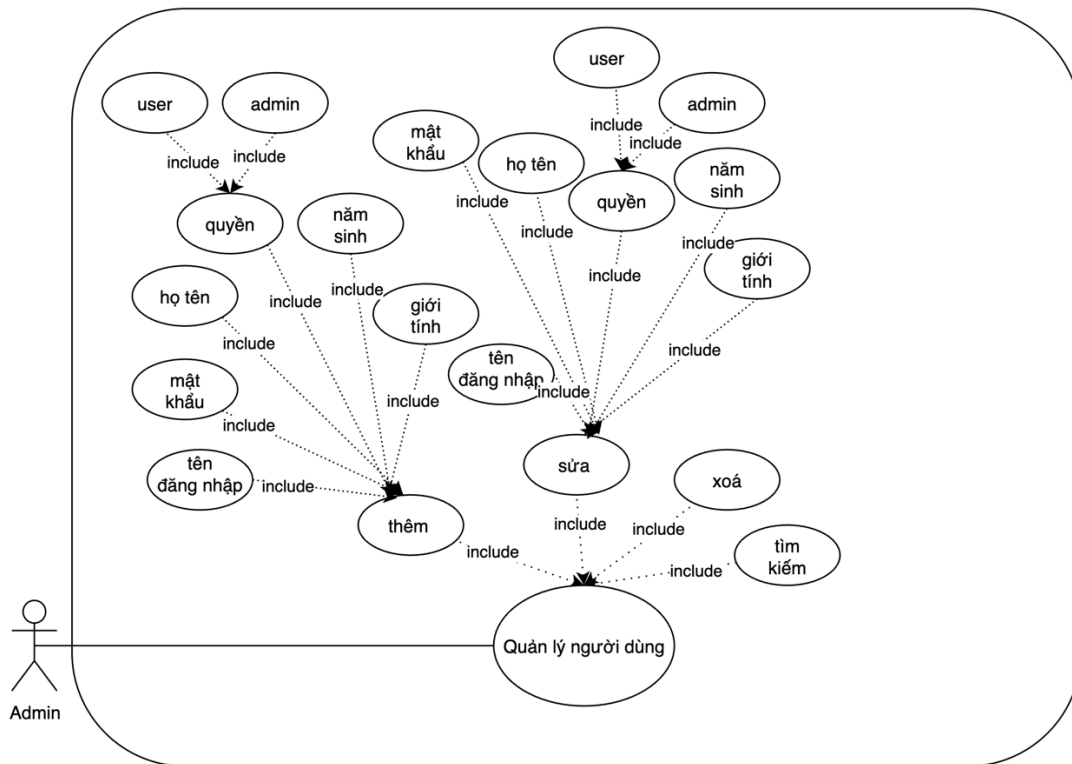
UC_QuanLyNguoiDung.
