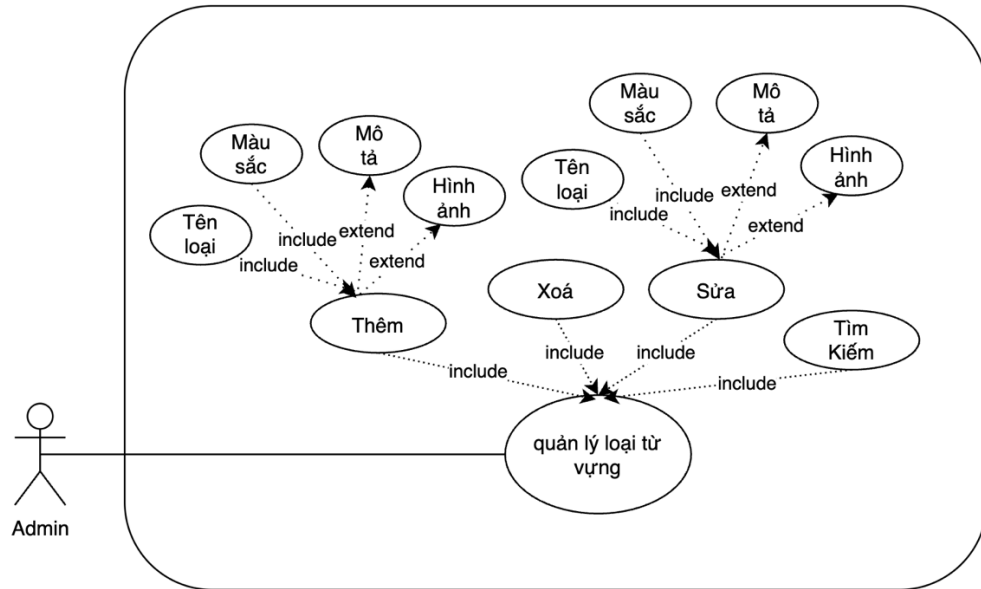
UC_WordTypeManagement.
