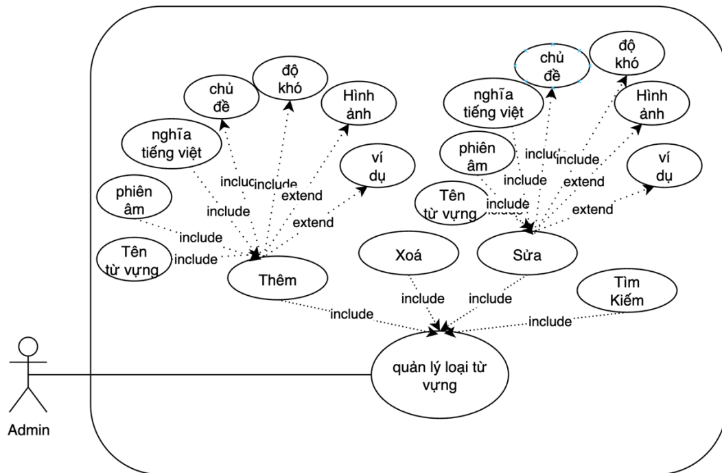
UC_VocabularyManagement.
