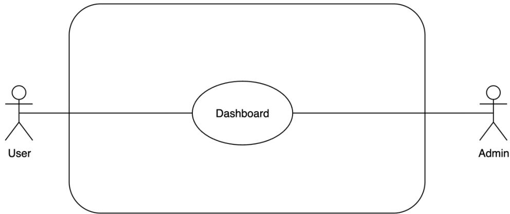
UC_Dashboard
