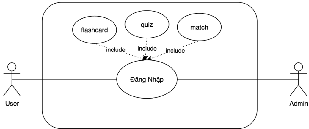
UC_Learn
