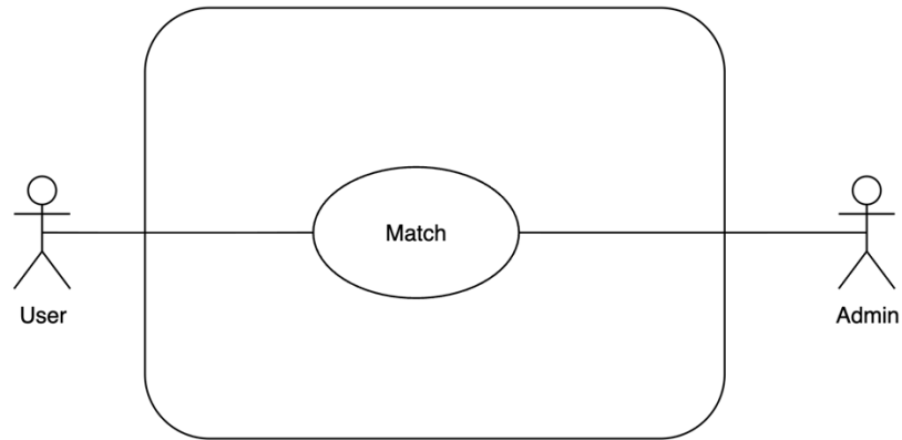
UC_Match.
